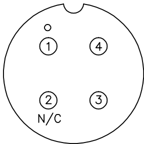
'FIXED' PLUG ON RECEIVER (VIEWED FROM FRONT)
