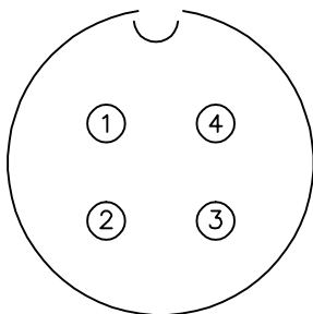
'FREE' SOCKET FROM MUTE PLUG TO RECEIVER HEAD (VIEWED FROM REAR)
